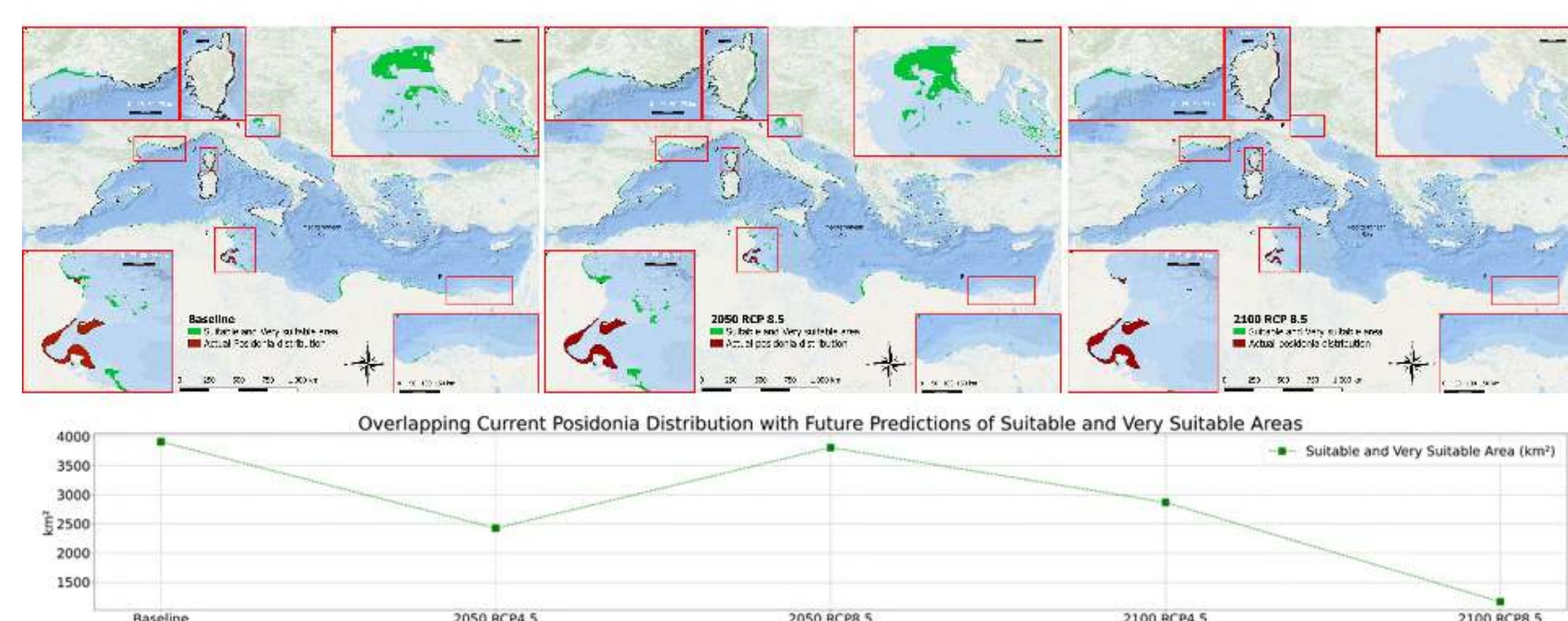
The figure showcases Overlapped maps with the combined suitable and very suitable class areas with the current distribution of P. oceanica (top panel) and line plot (bottom panel) for the area changes comparing the baseline to future scenarios (2050 RCP 4.5, 2050 RCP 8.5, 2100 RCP4.5, and 2100 RCP 85).
