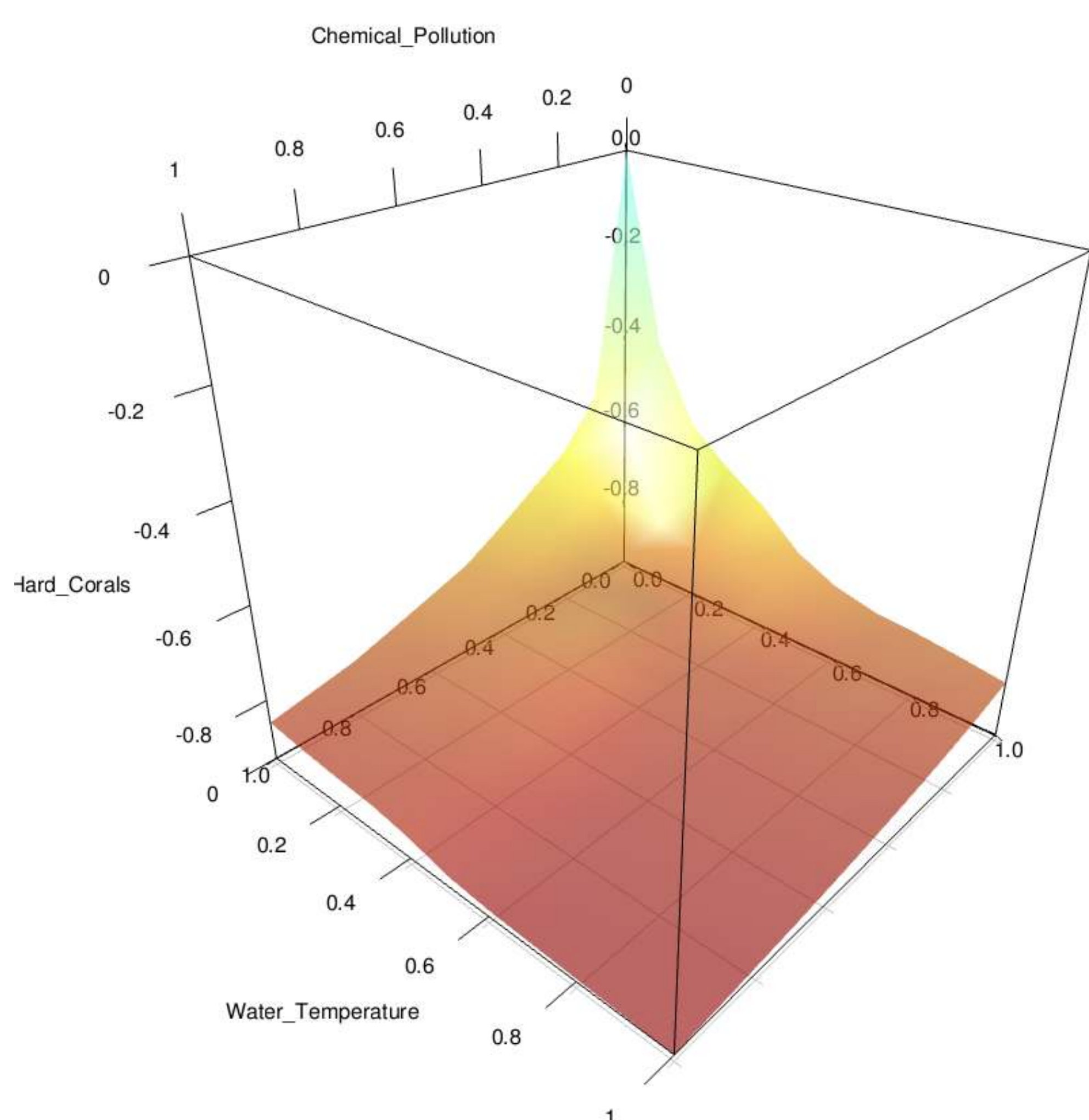
Effect of combined increase in water temperature and chemical pollution on hard corals from the coral reefs conceptual model.
