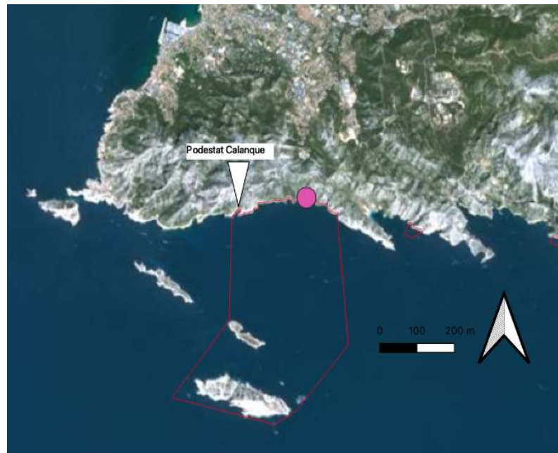
Figure 4. France Case Study (Northwestern Mediterranean) showing the location of the sampling site that has been surveyed with underwater fish censuses for 9 years (white arrow). The pink dot shows the location of the outflow pipe from the wastewater treatment plant. The red line indicates a No-take area of the National Park of Calanques.
