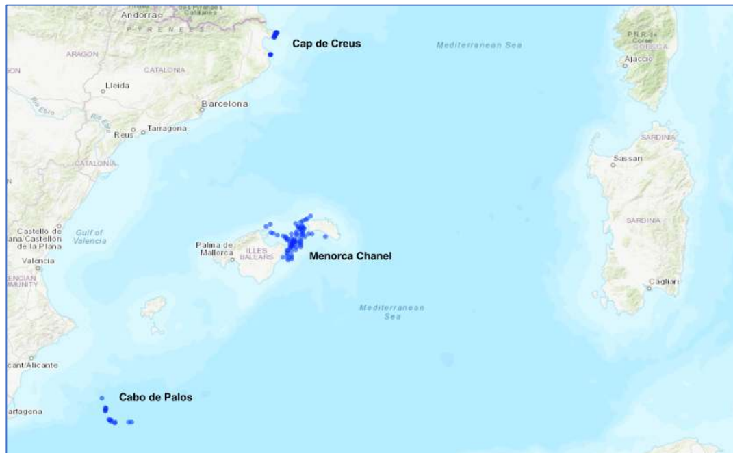
Figure 8. Maërl beds in the Spanish case study, Northwestern Mediterranean: Cabo de Palos, Cap de Creus and Menorca Channel. Blue dots indicate the sampling sites.
